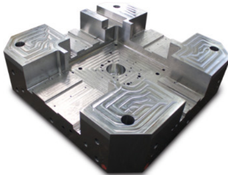
MOLD PLATES
